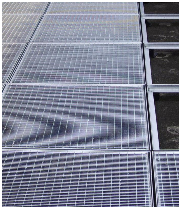
Fig. 12: PLV50/75 combined with ZSt65/100, supporting grid, 135-170 mm.
