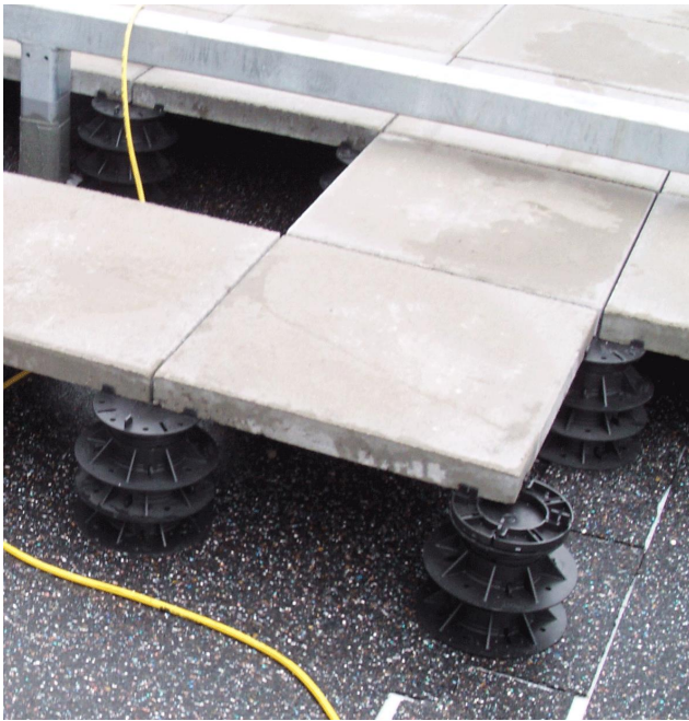
Fig. 7: Height adjustable PLV50/75 combined with PP155/15, Project „euro-gate“ Hamburg.
