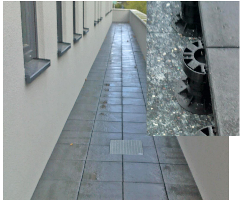
Fig. 10: Project GIG Hohenzollernring, Münster PLV50/75, ZSt65/100, PP155/15 and AS15/3.
